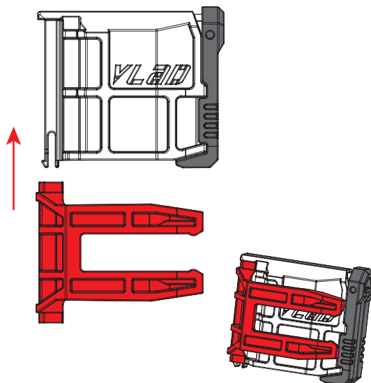
STEP 3-2 Left side mount
